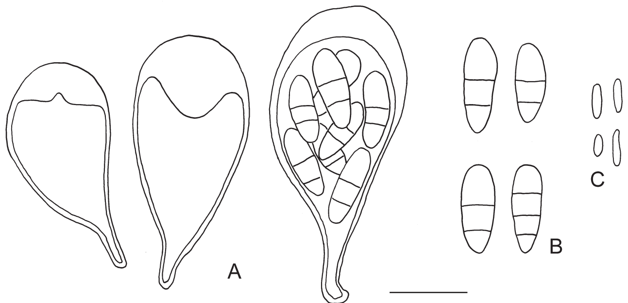
Fig. 2. Inoderma applanatum anatomy. A Non-amyloid asci, with young asci on left and mature, 8-spored ascus on right. B Ascospores. C Conidia. Scale bars = 10 \mu\text{m} .
