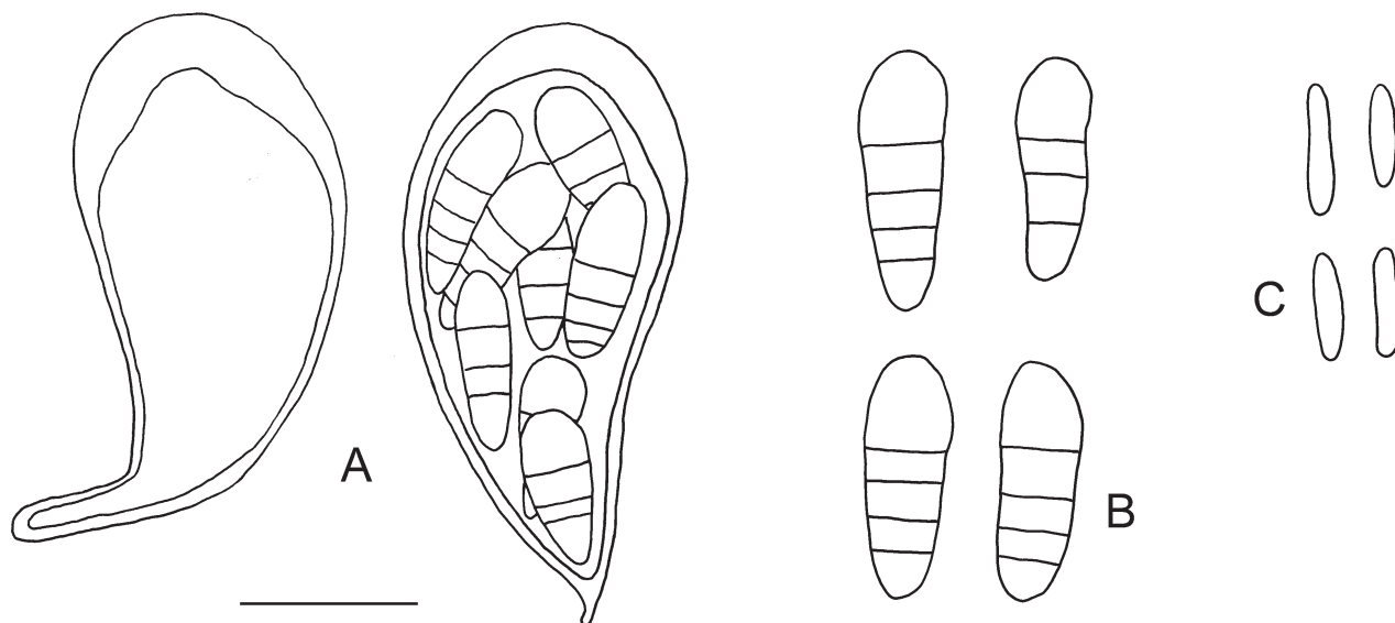
Fig. 4. Inoderma platygraphellum anatomy. A Non-amyloid asci, with young ascus on left and mature, 8-spored ascus on right. B Ascospores. C Conidia. Scale bars = 10 \mu m.
