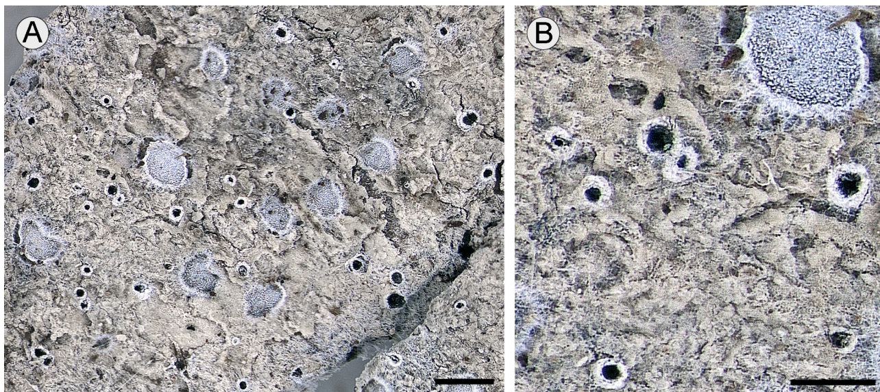
Fig. 3. Inoderma platygraphellum morphology. A Plane, adnate, thickly pruinose apothecia with a whitish rim, and semi-immersed pycnidia with black ostioles. B Detail of pycnidia. Scale bars: A = 1 mm, B = 500 \mu m. Photos: J. Jarman.
