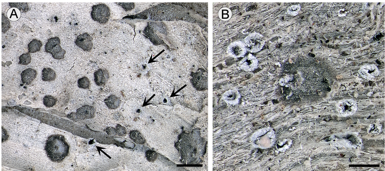
Fig. 1. Inoderma applanatum morphology. A Plane, adnate, thinly pruinose apothecia and emergent pycnidia (arrows). B Detail of pycnidia. Scale bars: A = 1 mm, B = 500 \mu\text{m} . Photos: J. Jarman.
